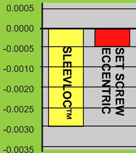
UNDERSIZED SHAFT ALLOWANCE COMPARISON-INCHES (for 1 15/16" Shafting)
